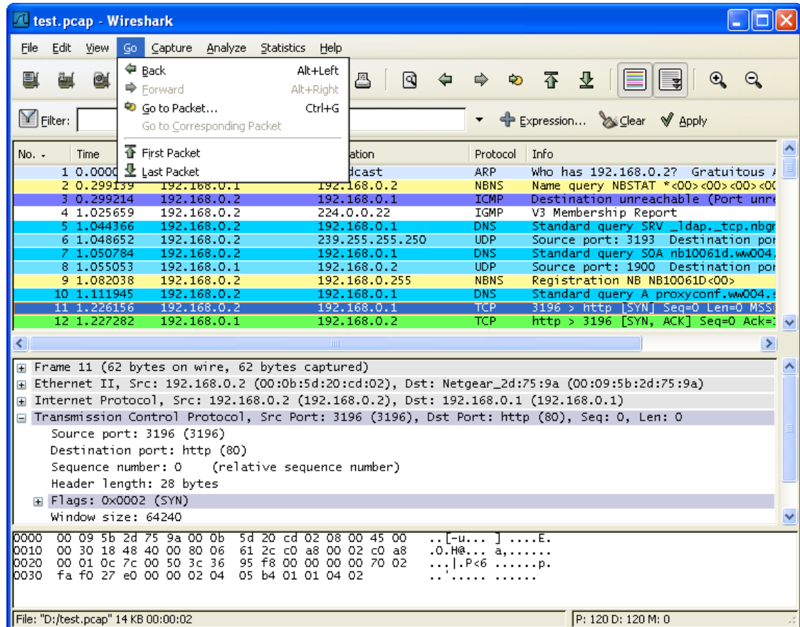
Figure 3.6. The "Go" Menu
