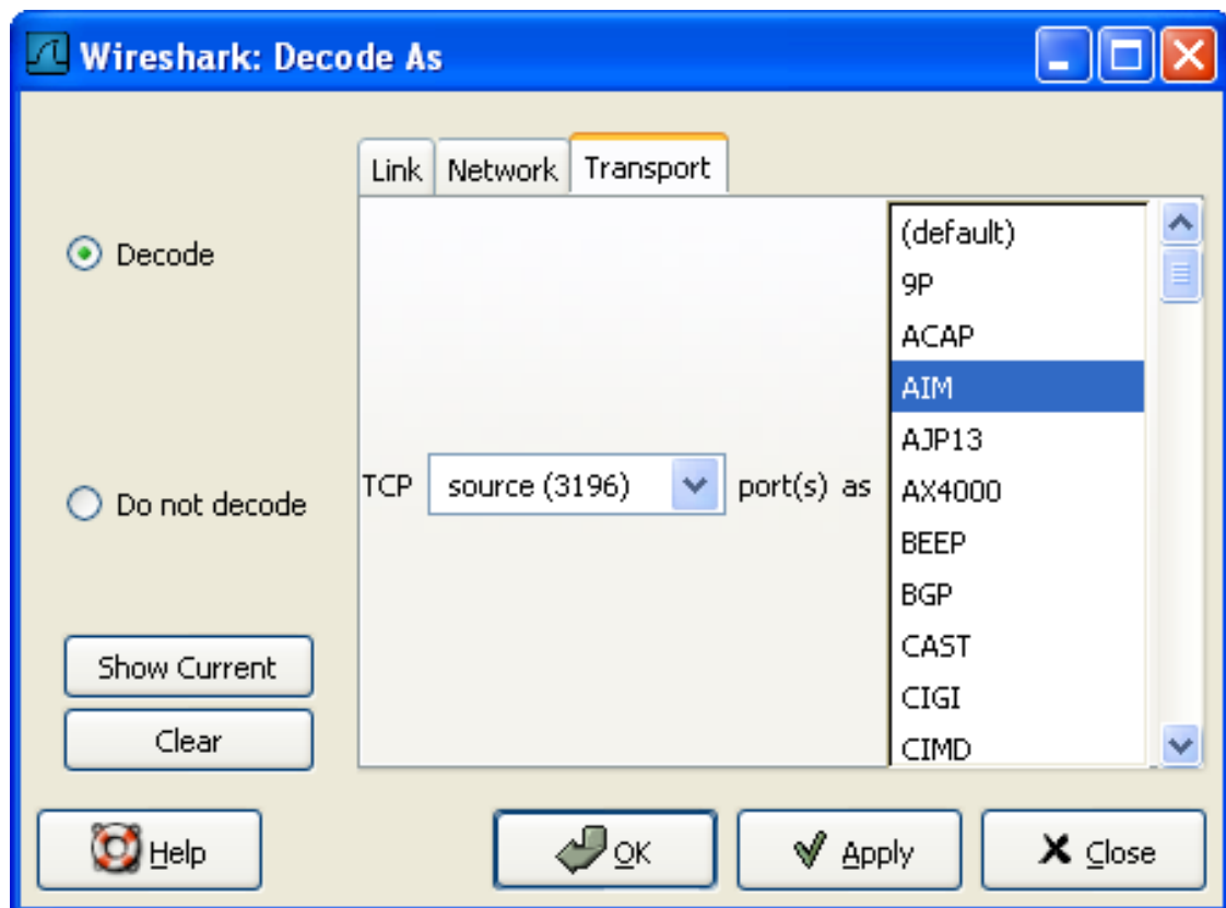
Figure 9.6. The "Decode As" dialog box
