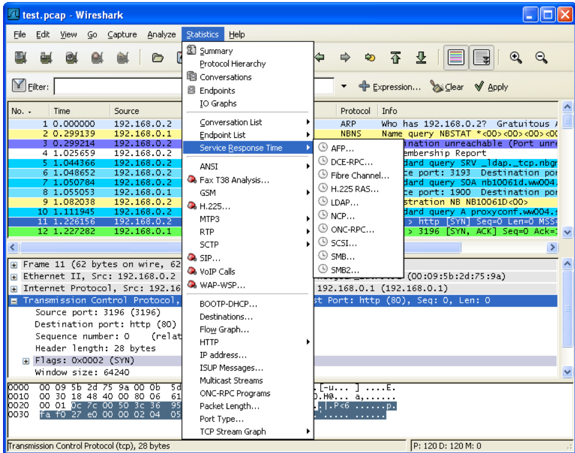
Figure 3.9. The "Statistics" Menu
