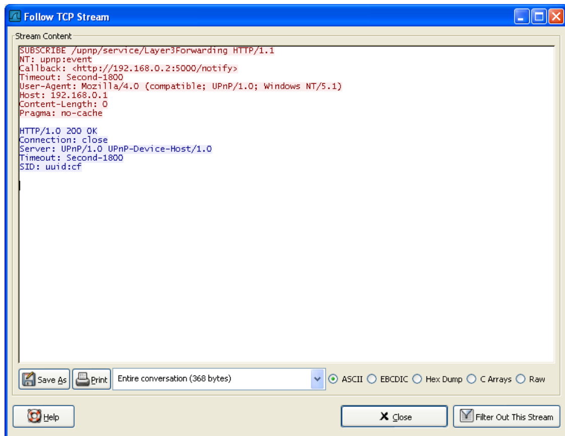
Figure 7.1. The "Follow TCP Stream" dialog box
