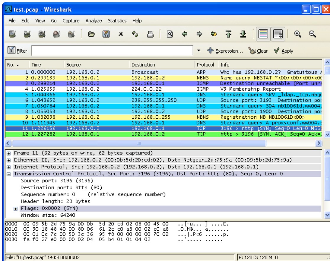
Figure 3.1. The Main window
