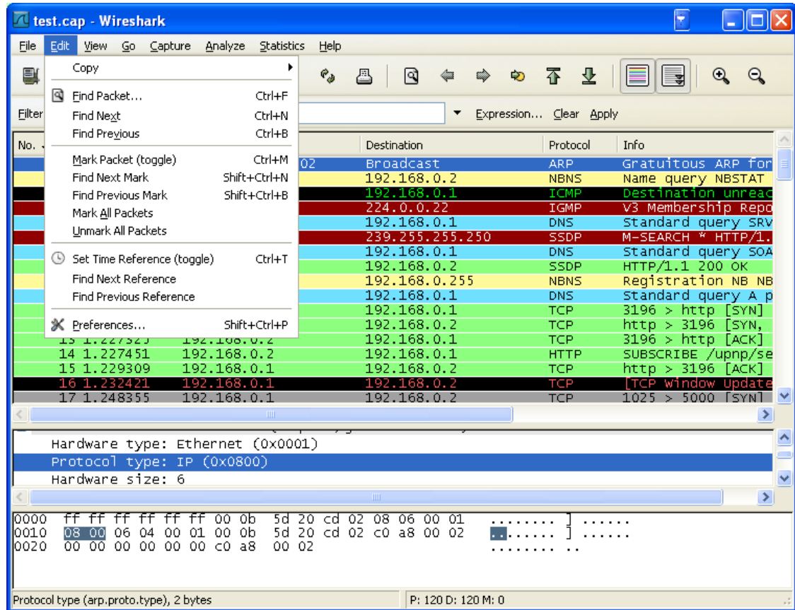
Figure 3.4. The "Edit" Menu
