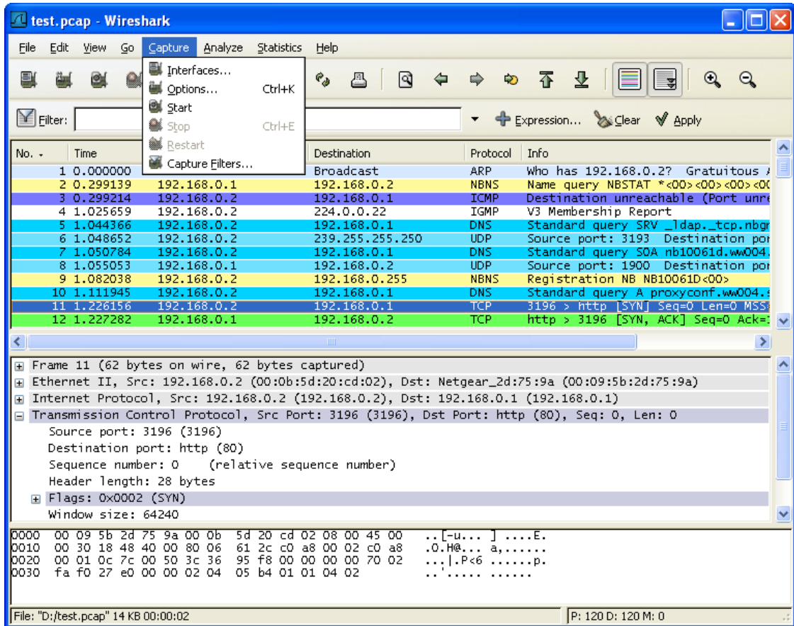
Figure 3.7. The "Capture" Menu
