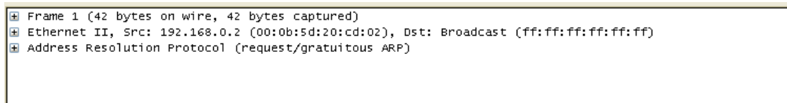
Figure 3.14. The "Packet Details" pane
