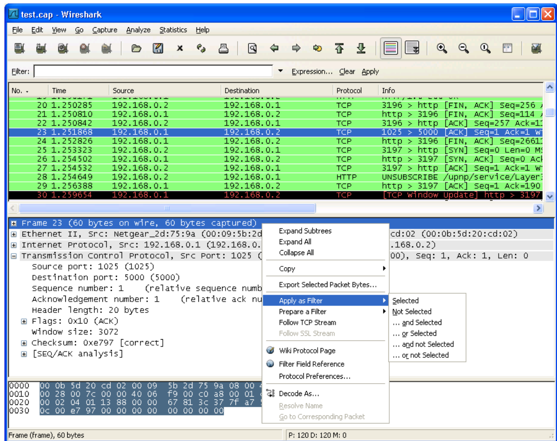
Figure 6.4. Pop-up menu of the "Packet Details" pane
