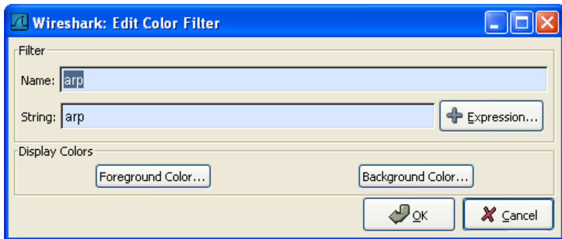
Figure 9.2. The "Edit Color Filter" dialog box
