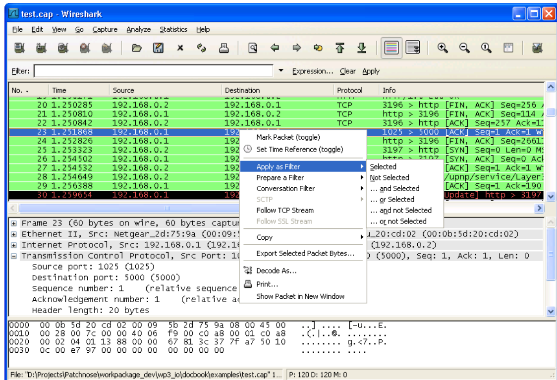
Figure 6.3. Pop-up menu of the "Packet List" pane
