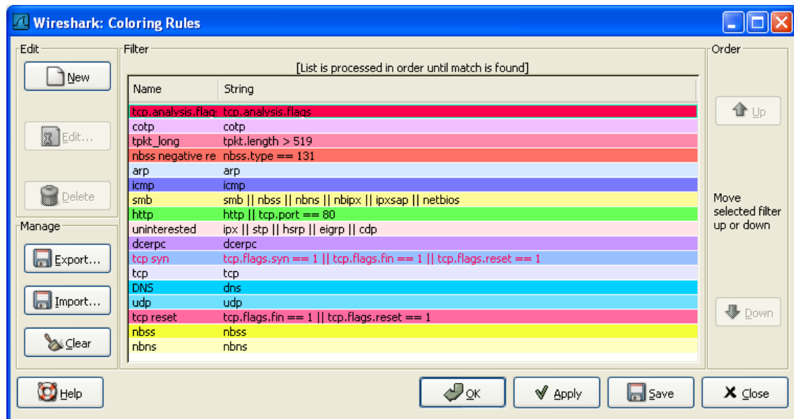
Figure 9.1. The "Coloring Rules" dialog box
