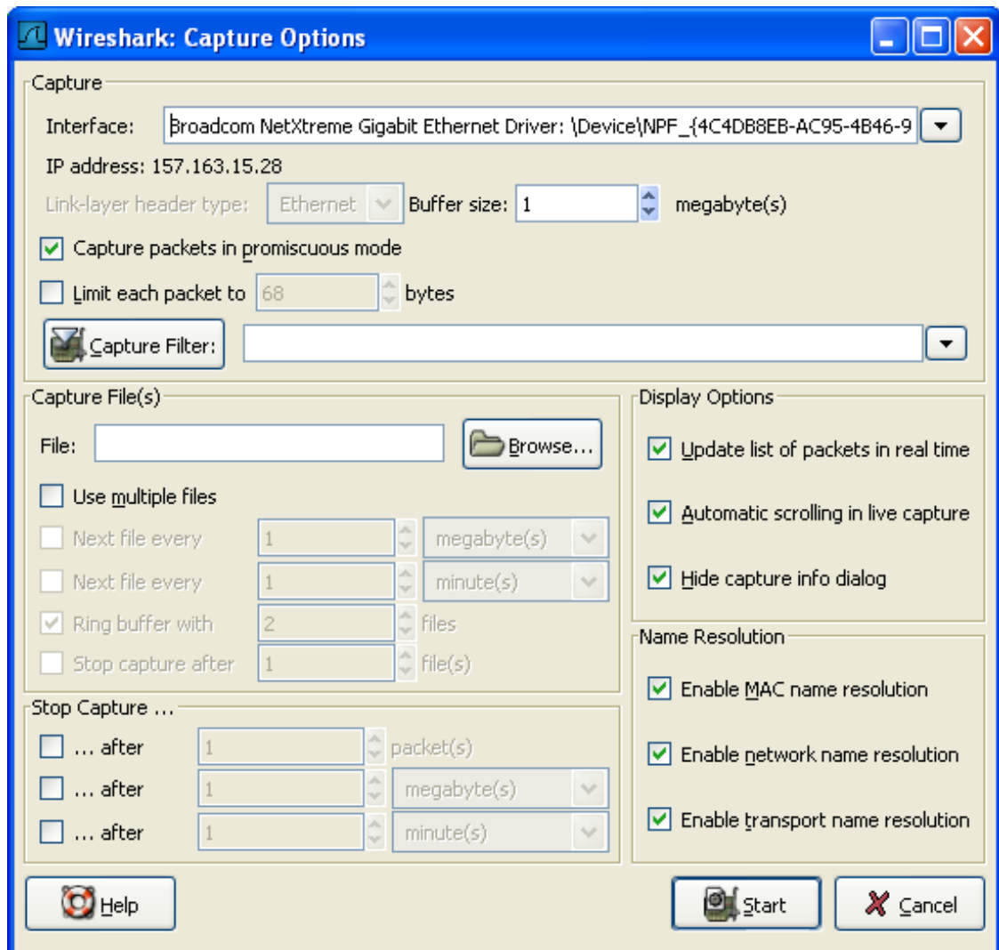
Figure 4.3. The "Capture Options" dialog box
