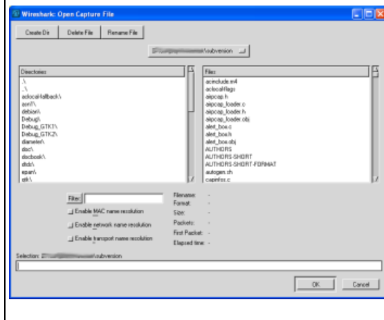
Figure 5.3. "Open" - old GTK version
