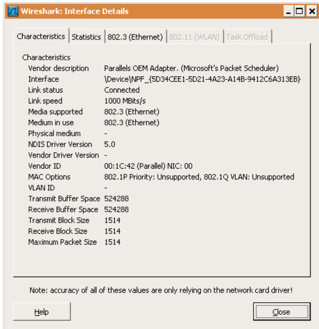
Figure 4.4. The "Interface Details" dialog box
