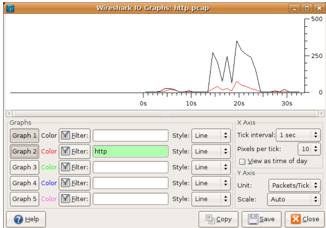
Figure 8.5. The "IO Graphs" window
