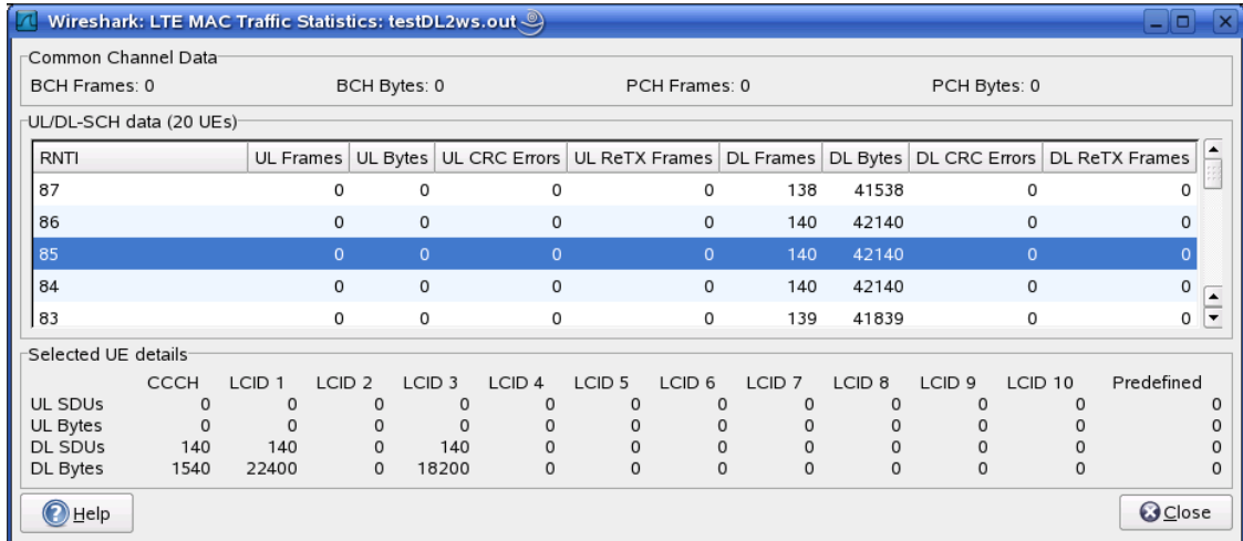
Figure 8.7. The "LTE MAC Traffic Statistics" window
