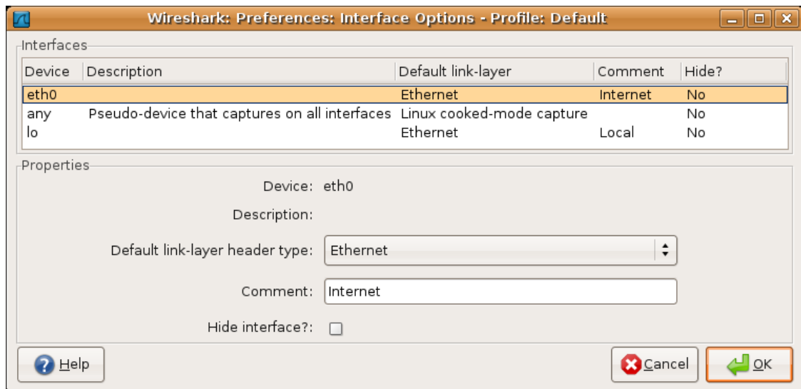
Figure 9.9. The interface options dialog box
