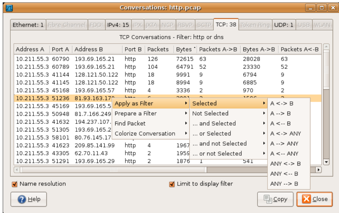
Figure 8.3. The "Conversations" window
